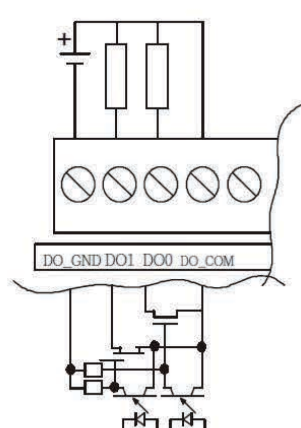
5188x-T/5189x-T Output
