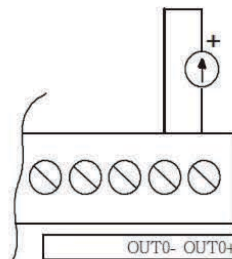
Current Output
