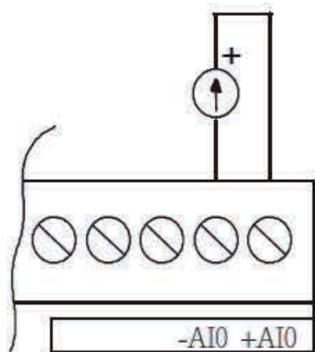
Current Input
