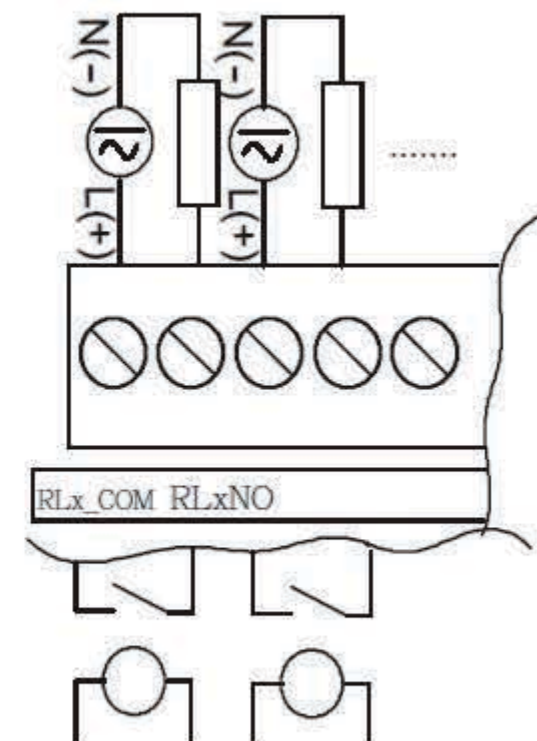
Relay Output
